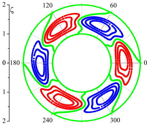
Figure 2: Flow in a gap. The unstable mode. Red, blue and green lines correspond to negative, positive and zero values of stream function.
