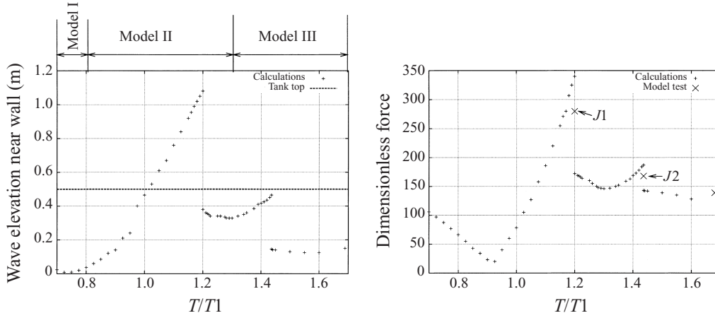
FIGURE 12. Wave elevation near the wall and dimensionless lateral force 1000F_x/(\rho g l^2 b) with respect to rotation axis vs. T/T1 . Rectangular tank with l = 1.0 m, h/l = 0.5 , \psi_0 = 0.2 rad. The measurements of lateral force were made by Olsen (1970, personal communication).
