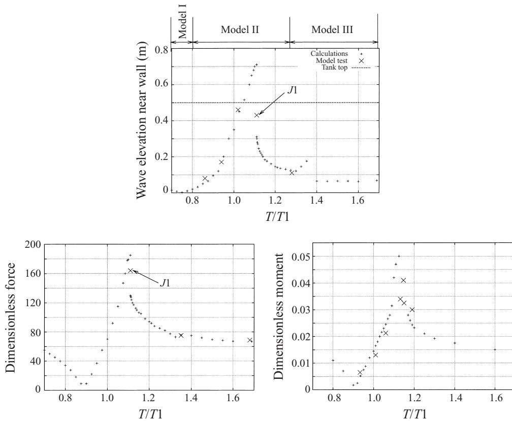
FIGURE 11. Wave elevation near the wall, dimensionless lateral force 1000F_x/(\rho g l^2 b) and dimensionless pitch moment M/(\rho g l^3 b) with respect to rotation axis vs. T/T_1 . Rectangular tank in figure 2(a) with h/l = 0.5 , \psi_0 = 0.1 rad. The measurements of lateral force and pitch moment were made by Olsen (1970, personal communication).
